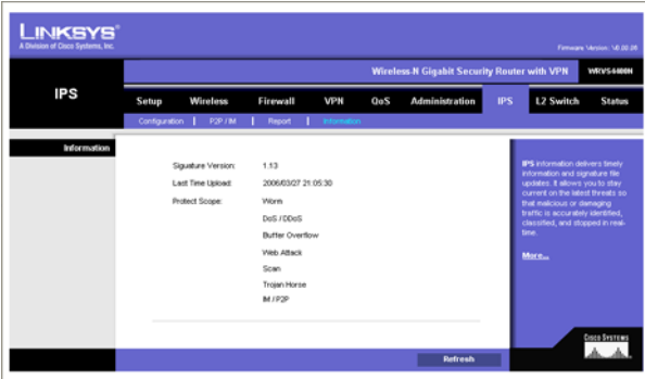
Figure 6-62: IPS - Information
